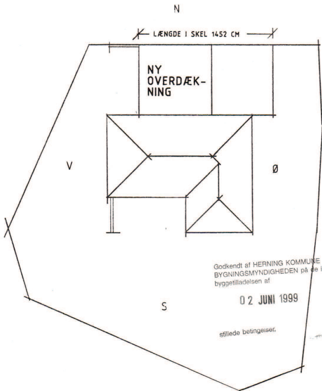
SITUATIONSPLAN 1:250.
